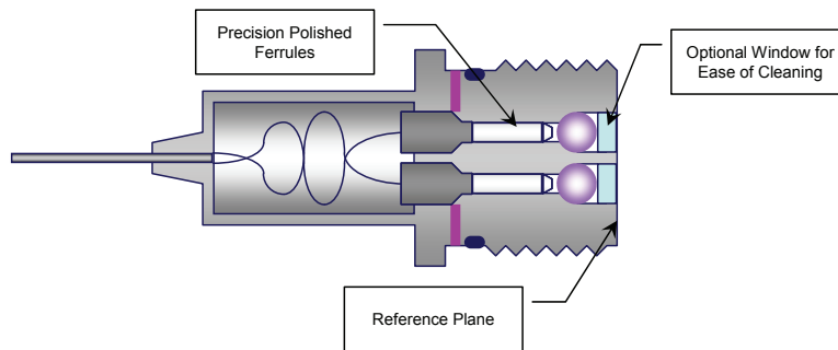
Figure 5. Schematic of multi-terminus EB connector showing optional windows for enhanced ease of cleaning and the reference plane for control of angular misalignment.
