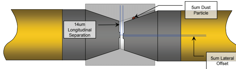
Figure 2. Minor contamination of biconic surfaces can lead to significant lateral and longitudinal offset and in turn, excess insertion loss.
