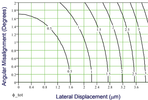
Figure 6. Insertion loss of single-mode optical connectors as a function of angular misalignment and lateral displacement.
