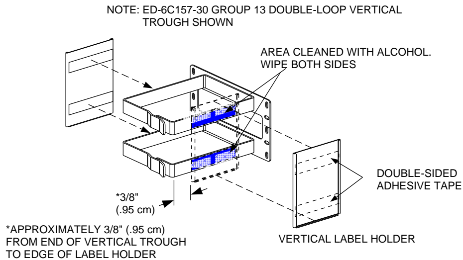
Figure 1. Vertical Label Holder Installation
