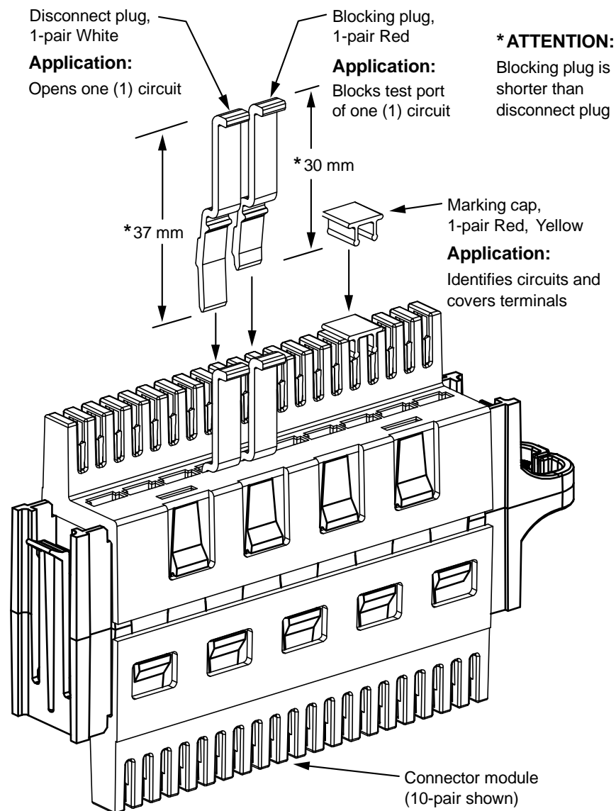
Figure 1. 1-Pair Disconnect Plug, Blocking Plug, and Marking Cap Instruction
