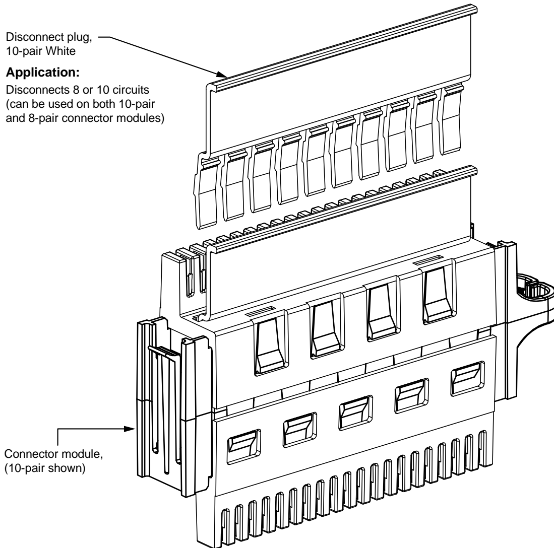
Figure 2. 10-Pair Disconnect Plug with Connector Module Instruction
