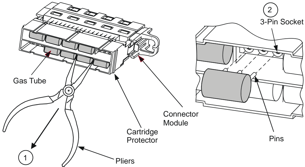
Figure 4. Removing and Installing Gas Tubes
