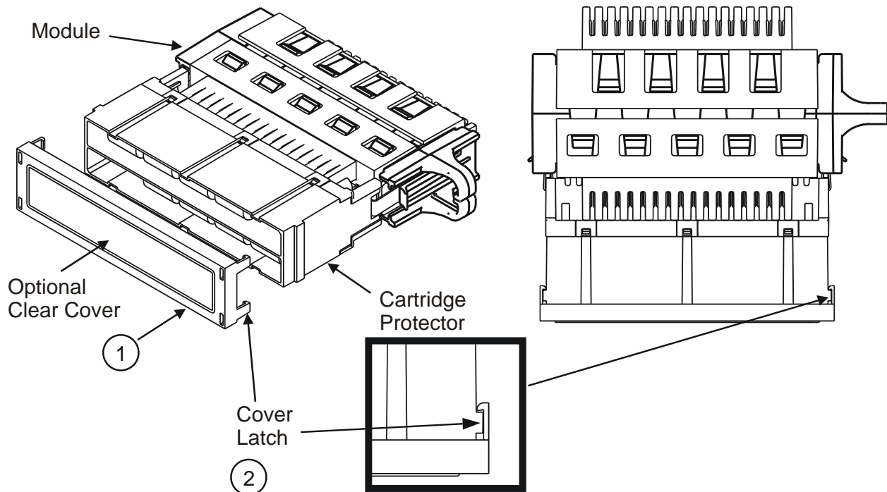
Figure 6. Installing and Removing Cover
