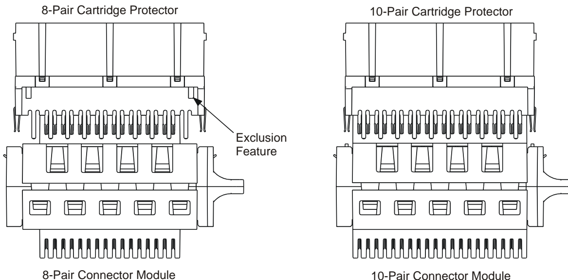
Figure 1. 8-pair Cartridge Protector on 10-pair Connector Module.
