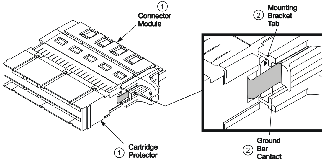
Figure 2. Installing Cartridge Protector
