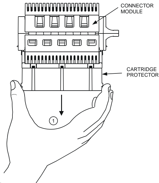
Figure 3. Removing the Cartridge Protector
