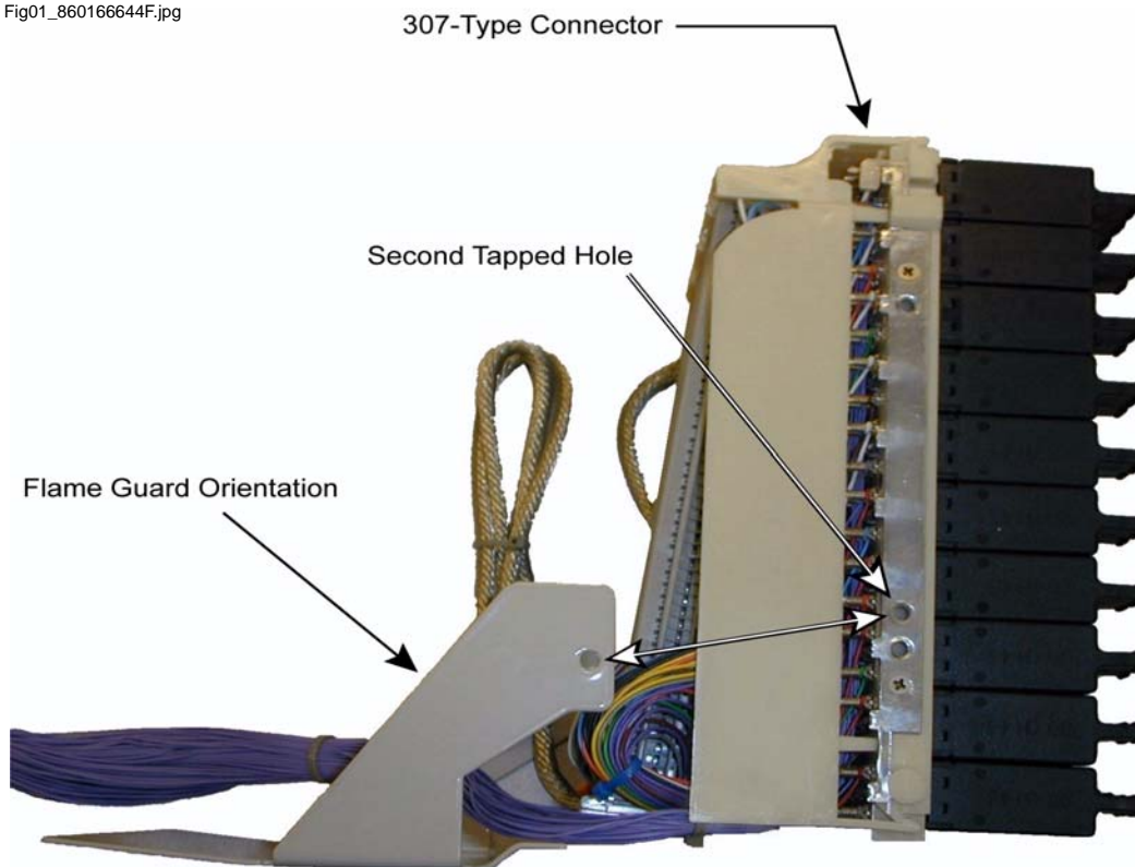
Figure 2. Positioning the Flame Guard for Installation
