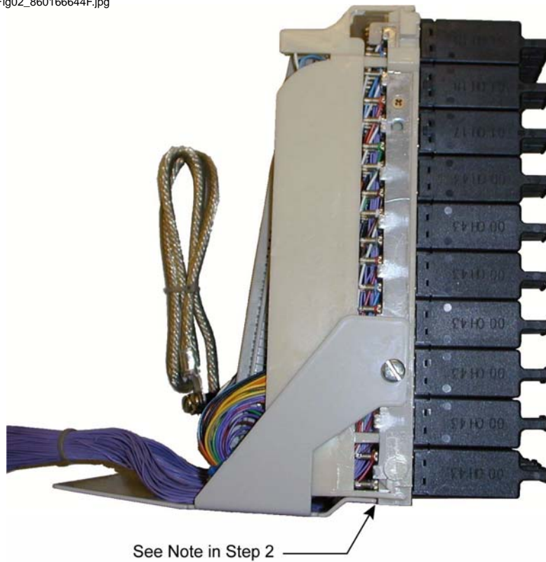
Figure 3. Installation of 307 Protector Panel Flame Guard
