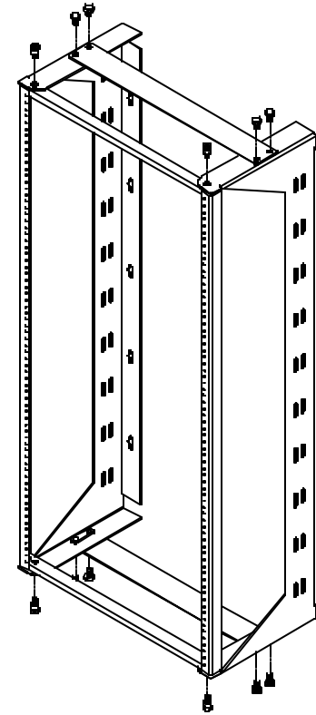
ISOMETRIC VIEW
