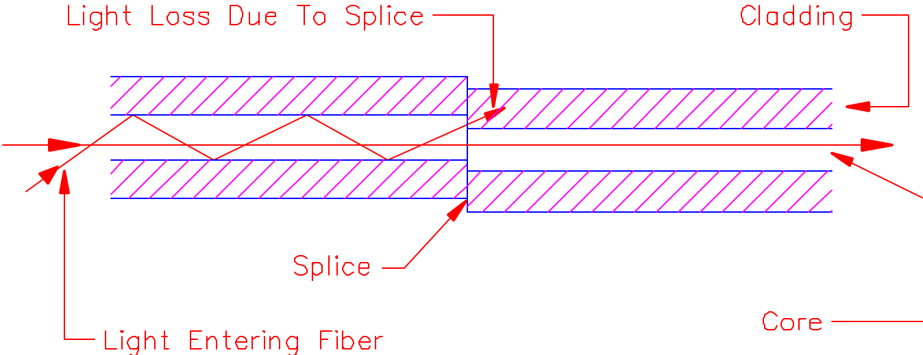
FIGURE 6 CORE MISALIGNMENT
